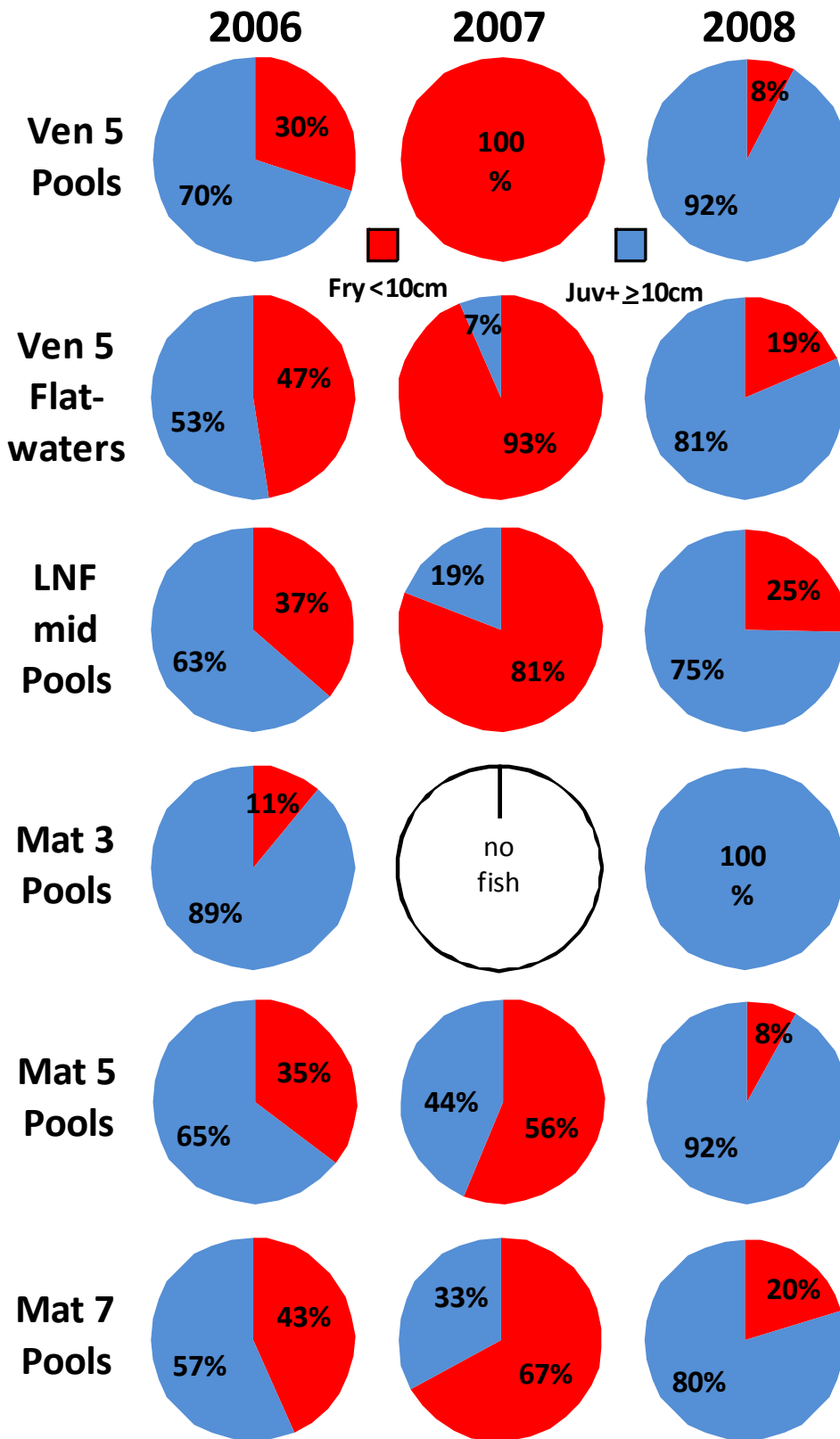
Figure 3. Relative proportion of O. mykiss fry and juvenile+ by year and study site.
