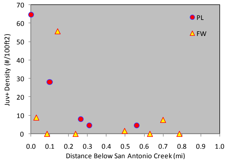
Figure 9. Relationship between distance from mouth of San Antonio Creek and density of juvenile+ O. mykiss in Ven 3 pool and flatwater habitat units.
