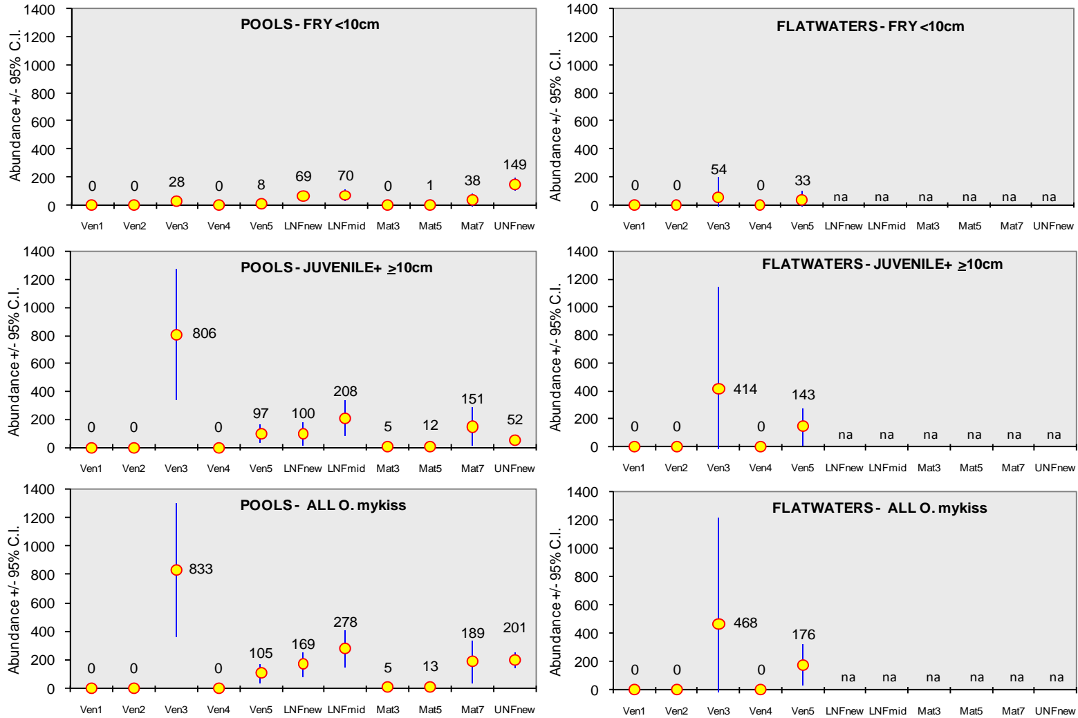
Figure 4. Estimated abundance of O. mykiss fry, juvenile+, and combined sizes according to study site and habitat type.
