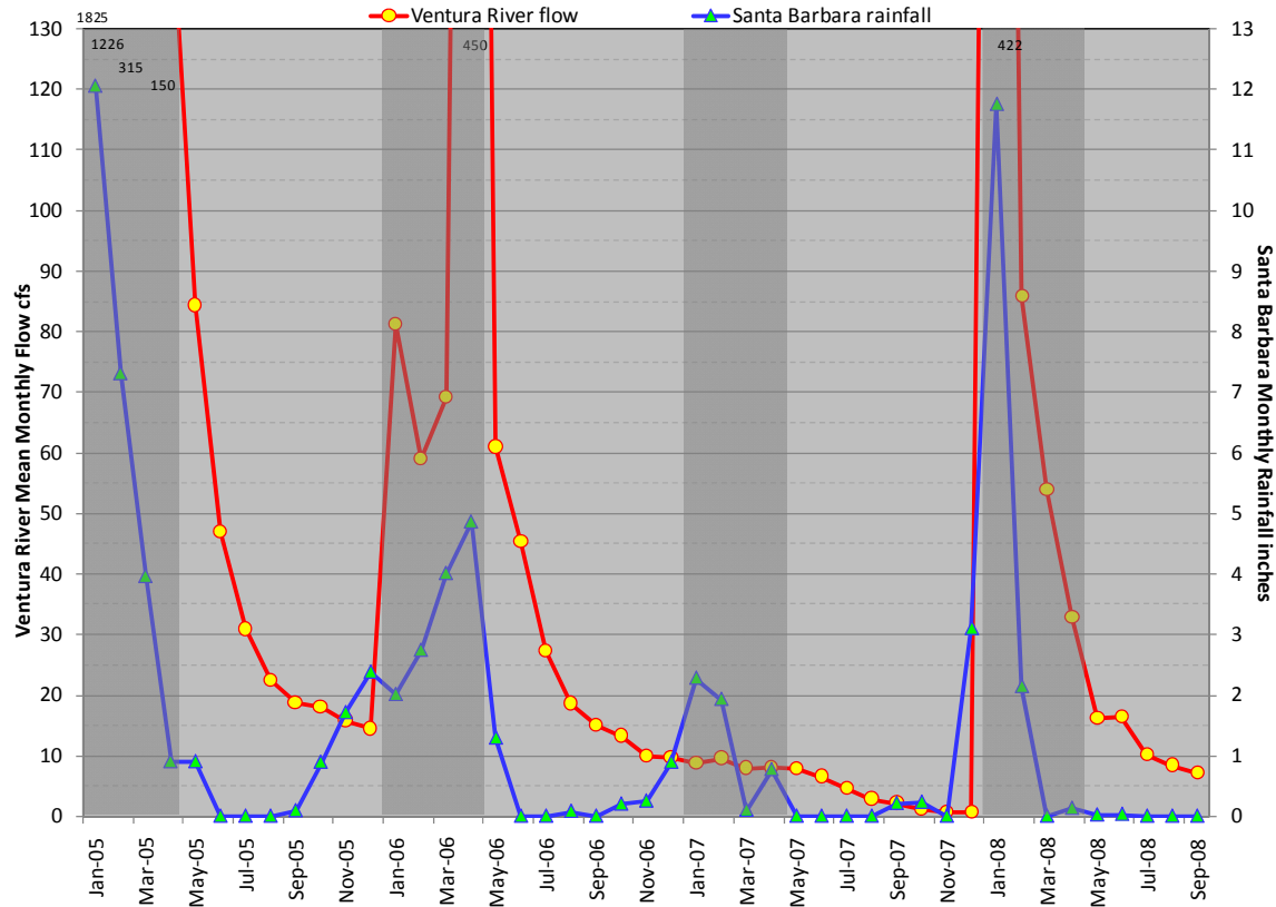
Figure 2. Mean monthly flows (cfs) in the Ventura River at Foster Park (USGS gage #8500) and total monthly rainfall at Santa Barbara (inches), 2005-2008. Shaded areas approximate the spawning and incubation periodicity for steelhead and rainbow trout.
