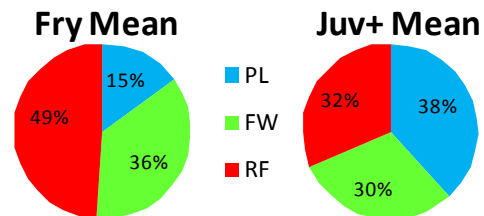
Figure 8. Mean relative proportion of O. mykiss fry ( <10 cm) and juvenile+ ( \geq 10 cm) found in pools, flatwaters, and riffles in 2006 and 2007, all study sites combined.
