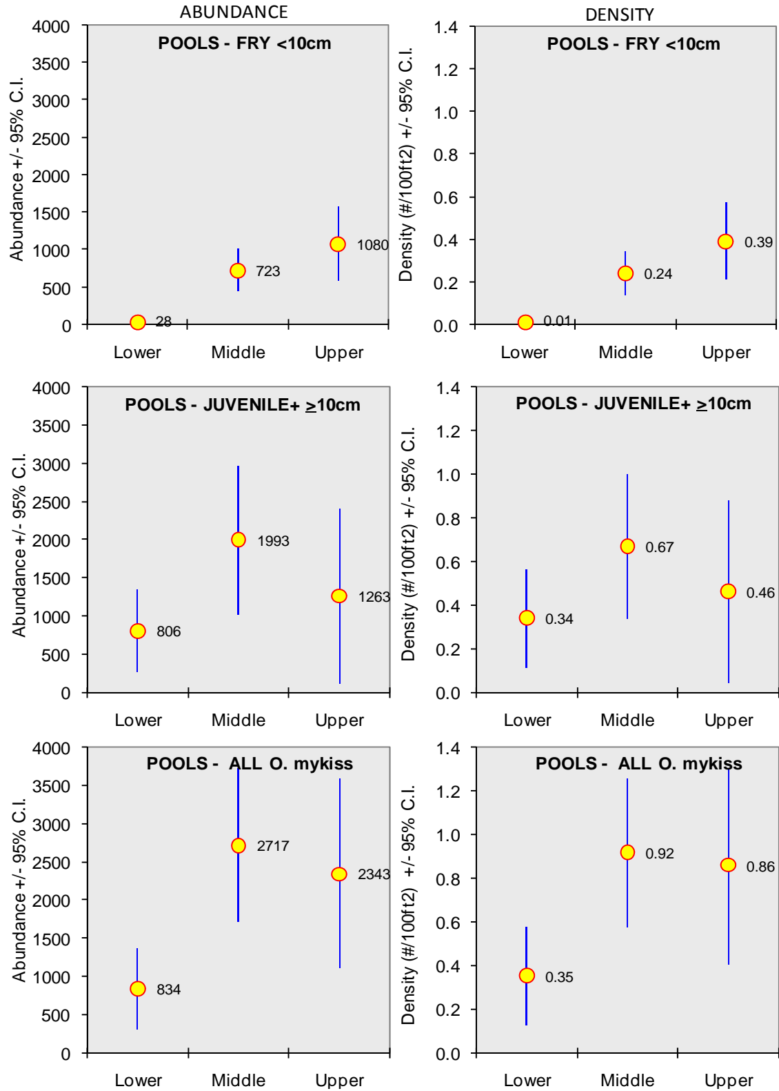
Figure 10. Estimated abundance and density of O. mykiss in pool habitats according to study segment in 2008.
