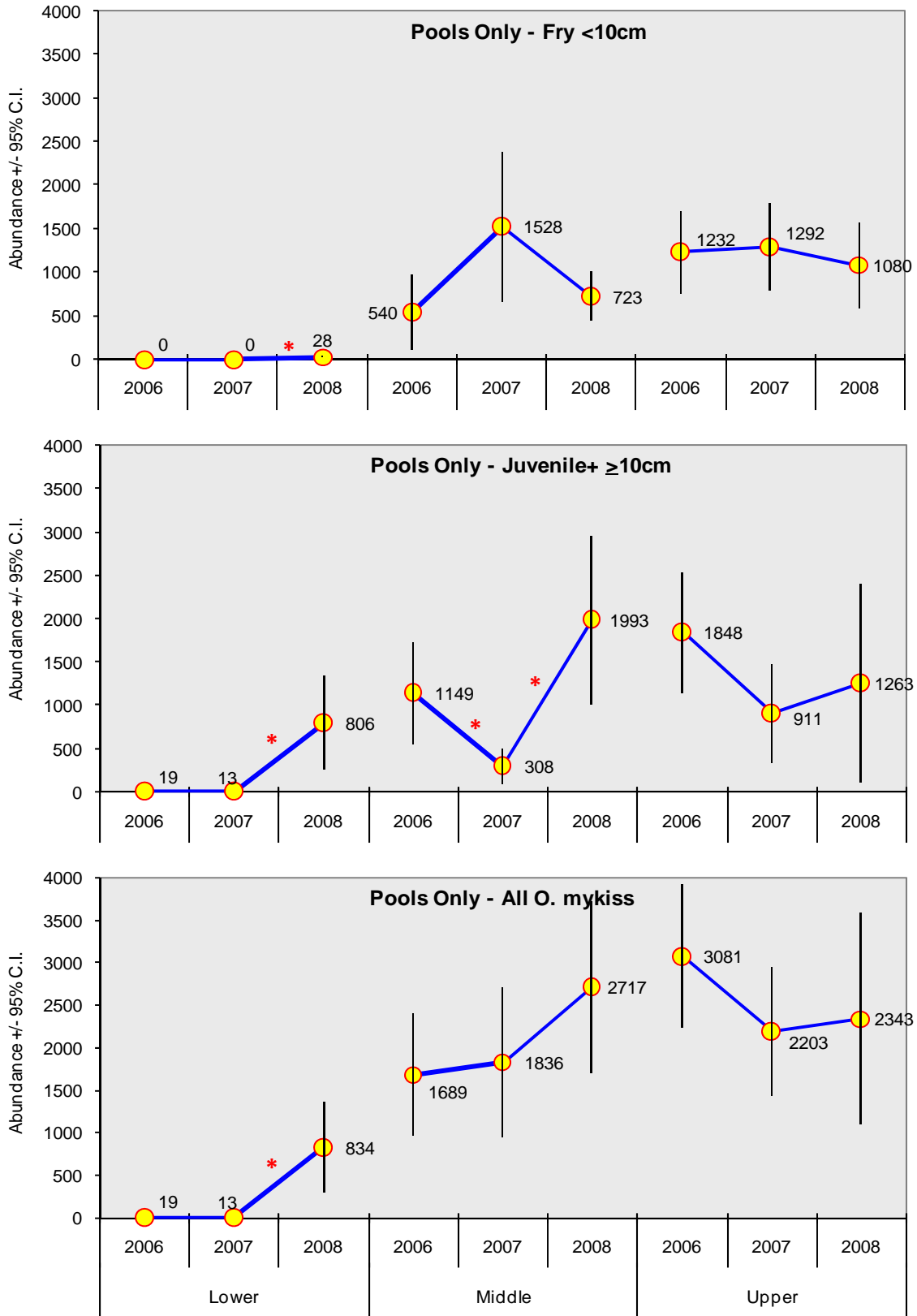
Figure 11. Estimated abundance of O. mykiss in pool habitats according to year and study segment. Asterisks indicate statistically significant differences between adjacent years.
