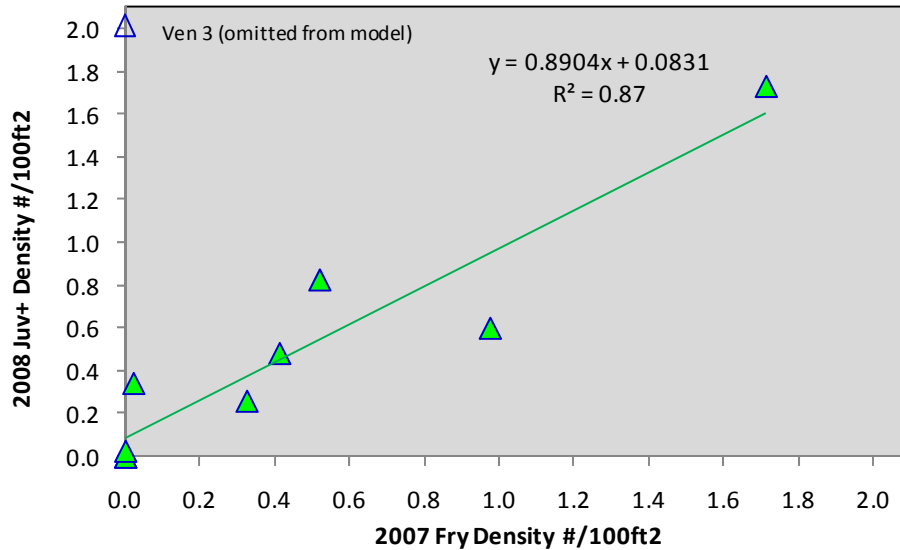
Figure 14. Relationship between densities of O. mykiss fry in 2007 and juvenile+ the following year, according to study site.
