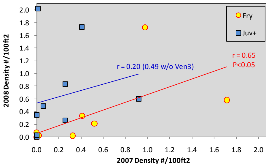
Figure 13. Correlation ( r ) in annual densities of O. mykiss by study site and size class.
