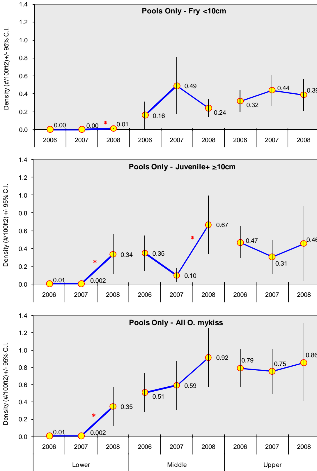
Figure 12. Estimated density (#/100ft 2 ) of O. mykiss in pool habitats according to year and study segment. Asterisks indicate statistically significant differences between adjacent years.
