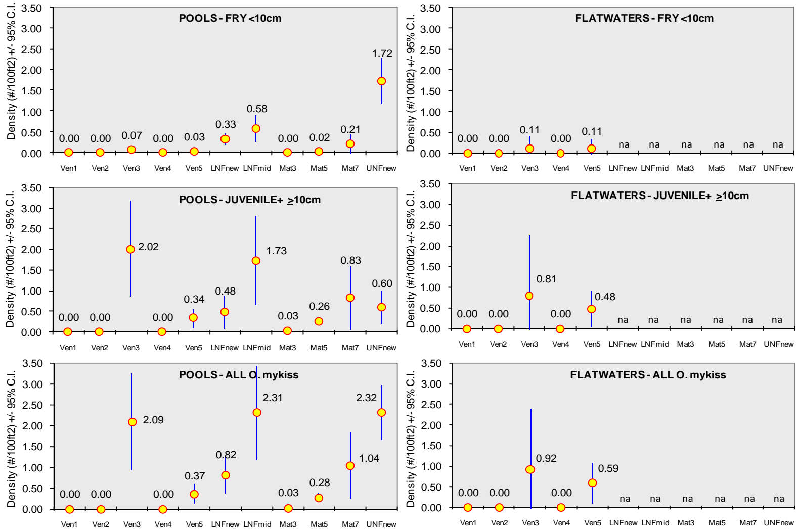
Figure 5. Estimated density (#/100ft 2 ) of O. mykiss fry, juvenile+, and combined sizes according to study site and habitat type.
